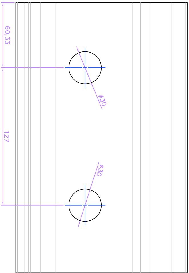
Fish Holes Dimensions Scale 1:2
