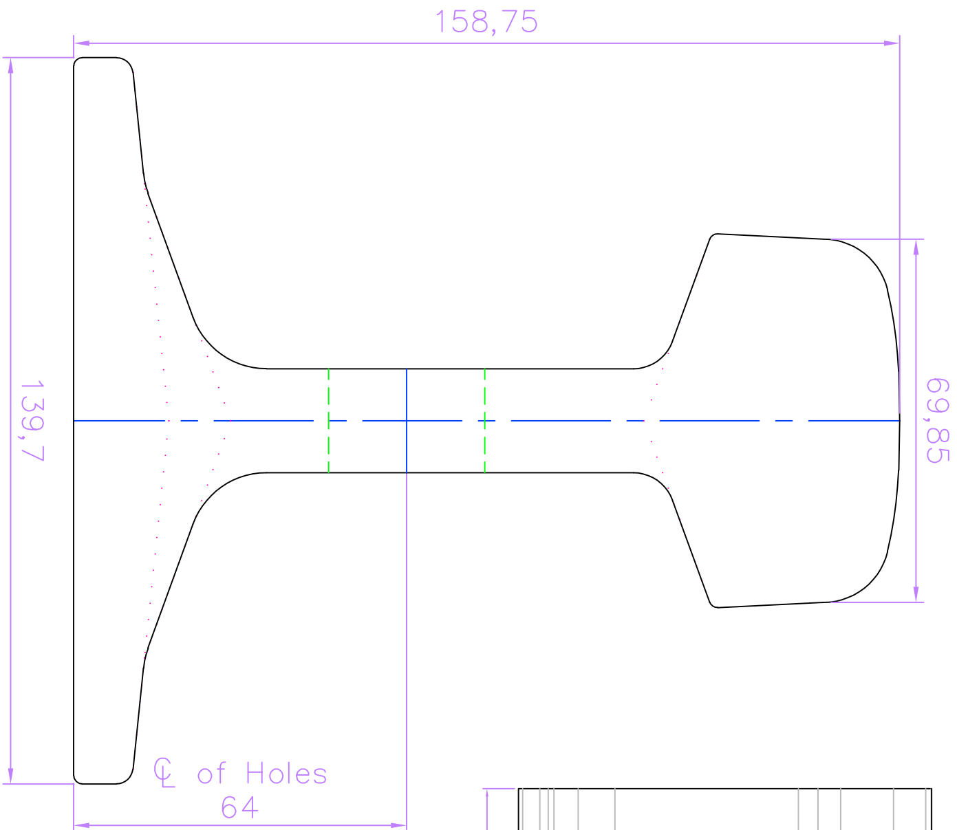
Profile Scale 1:1
