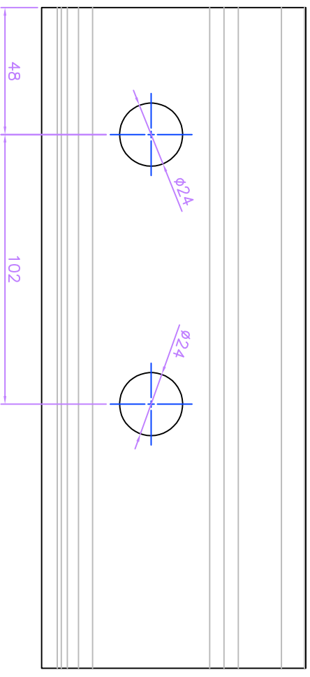
Fish Holes Dimensions Scale 1:2
